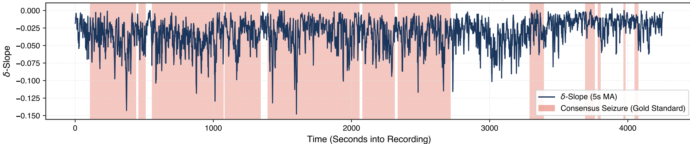
Patient 38 (Channel: Fp2-F4) - Continuous Trajectory Tracking
