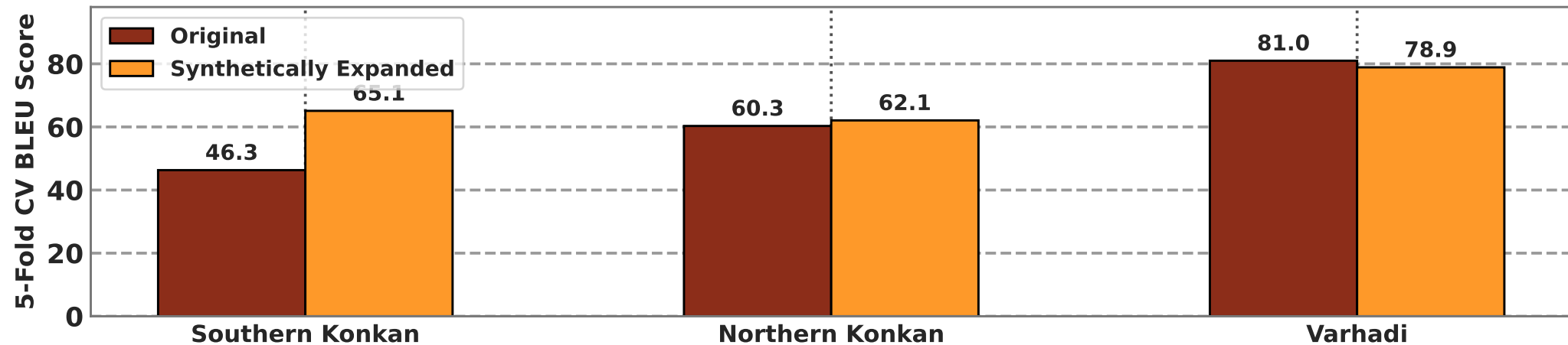
B. mT5-Small (300M) Single-Dialect CV BLEU
