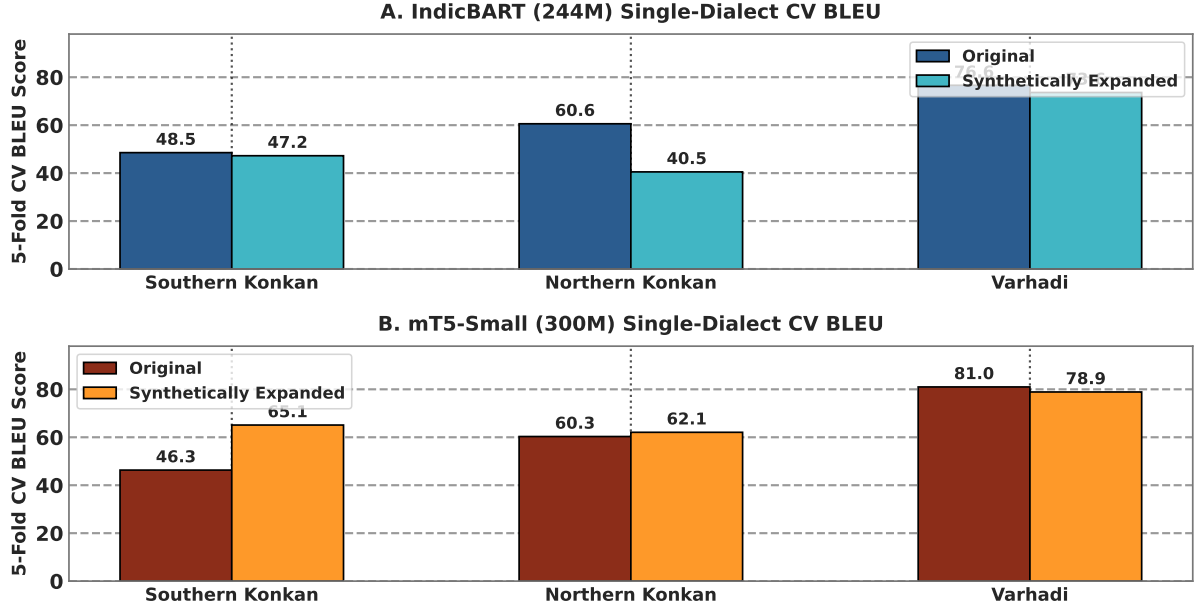
Figure 5: Single-dialect 5-fold cross-validation performance shift comparing Original and Synthetically Expanded models for IndicBART (244M) and mT5-small (300M).
