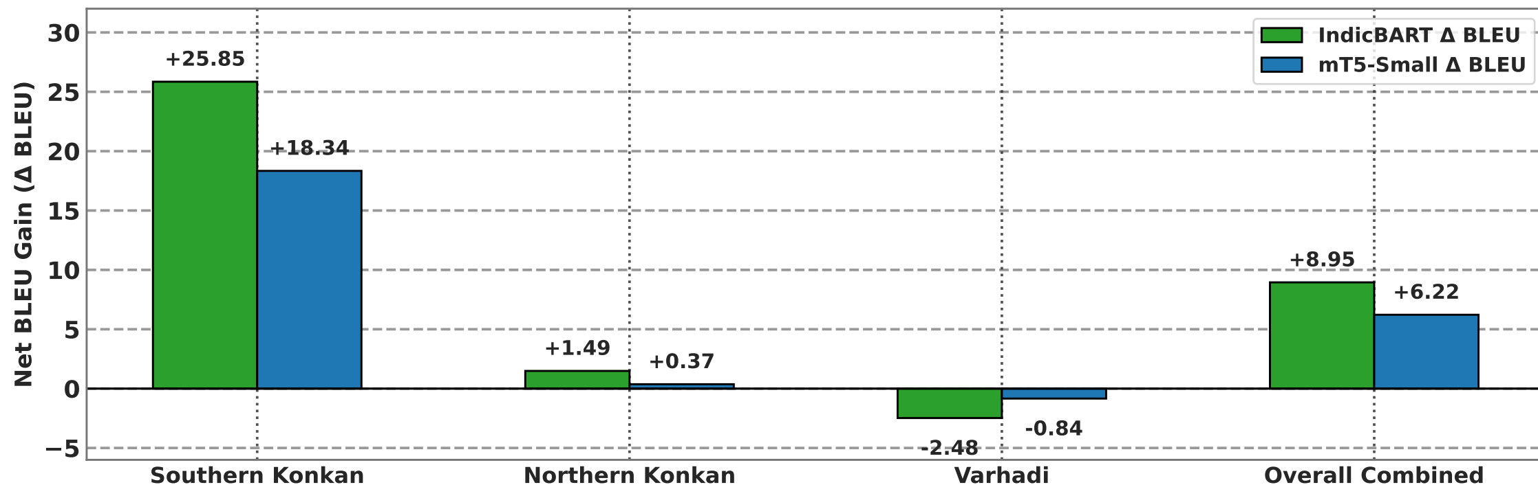
B. Synthetic Expansion Net Impact Across Dialects & Overall
