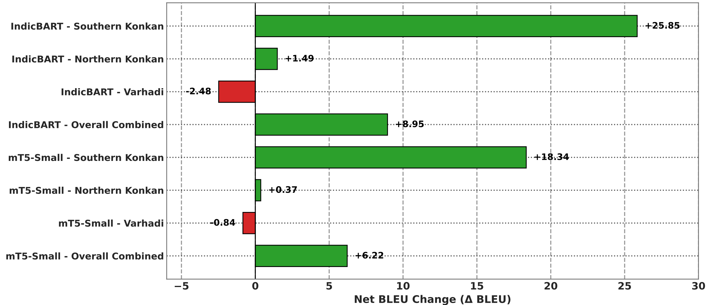
Impact of Synthetic Data Augmentation Across Models and Dialects
