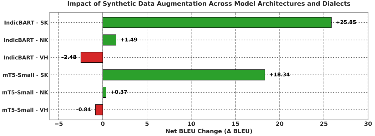
Figure 7: Impact of LLM synthetic data expansion ( \Delta BLEU score comparing synthetically expanded vs. original 5-fold cross-validation benchmarks).
