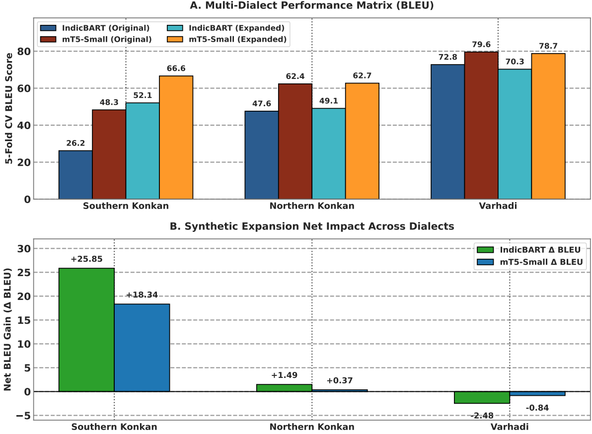
Figure 6: Multi-dialect 5-fold cross-validation benchmark comparison: (A) Absolute BLEU scores across model architectures and corpora partitions, and (B) Net synthetic expansion impact ( \Delta BLEU across sub-dialects).
