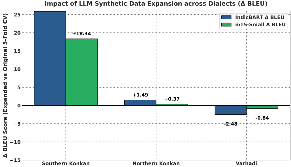
Figure 6: Impact of LLM synthetic data expansion ( \Delta BLEU score comparing synthetically expanded vs. original 5-fold cross-validation benchmarks).
