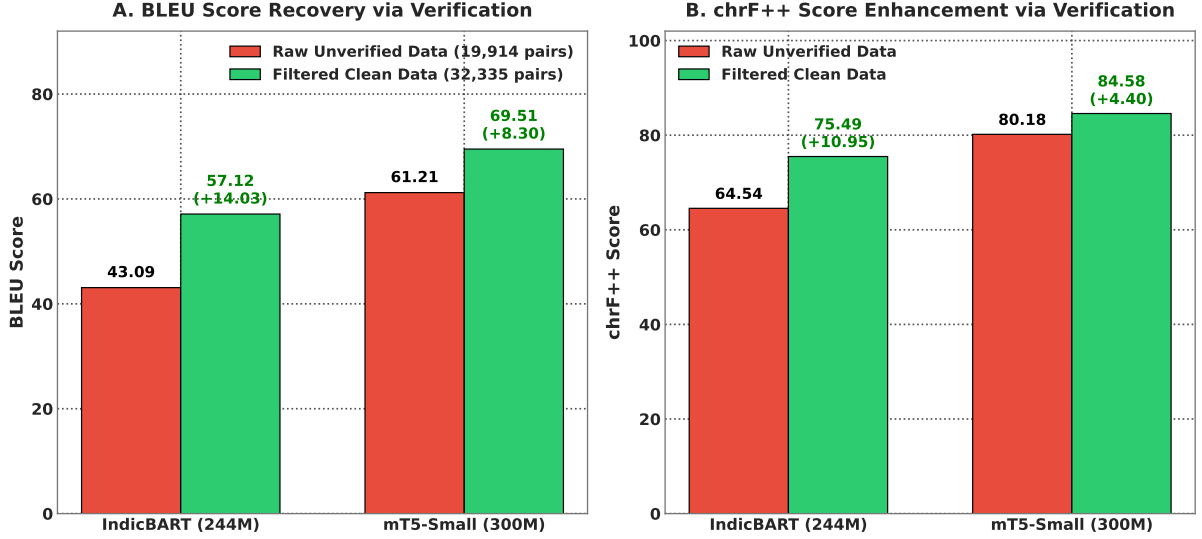
Figure 7: Multi-tier verification engine ablation: (A) BLEU score recovery and (B) chrF++ score enhancement comparing models trained on raw unverified synthetic outputs vs. filtered clean synthetic data.
