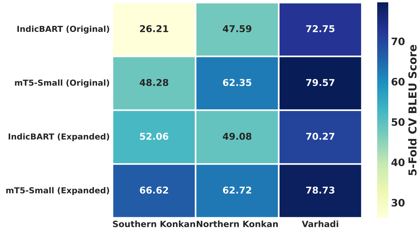
A. Multi-Dialect Performance Heatmap (BLEU)
