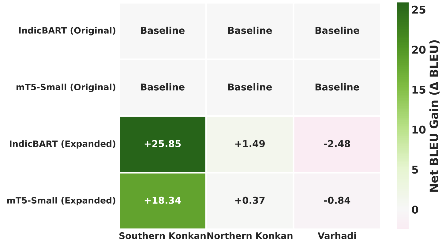
B. Synthetic Expansion Net Impact ( \Delta BLEU)
