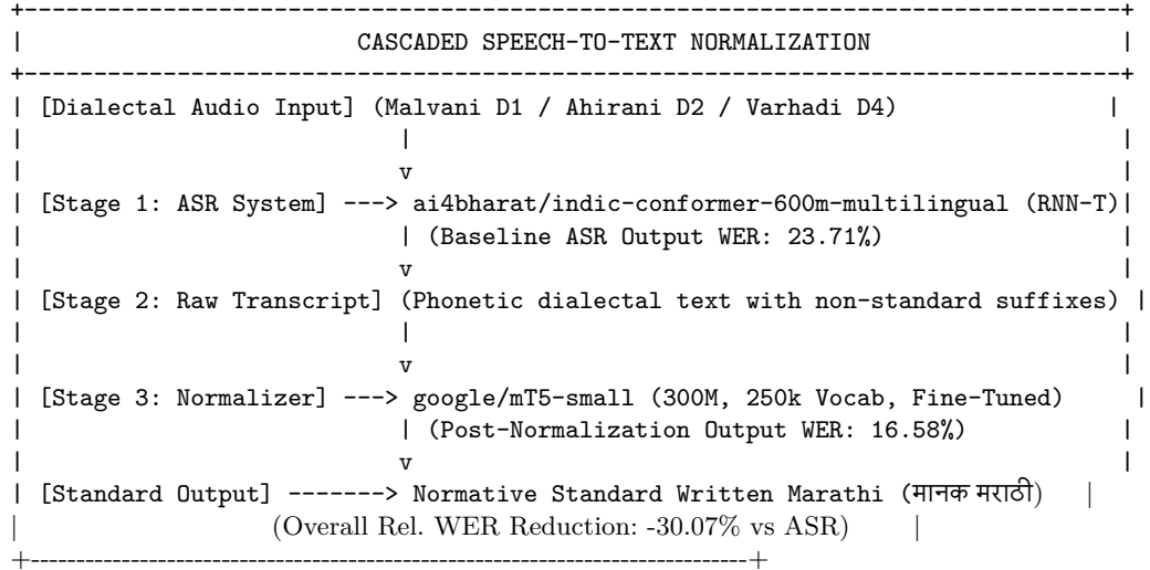
Fig. 1. Cascaded Architecture: Linking Acoustic ASR Transcriptions with Sequence-to-Sequence Text Normalization.
