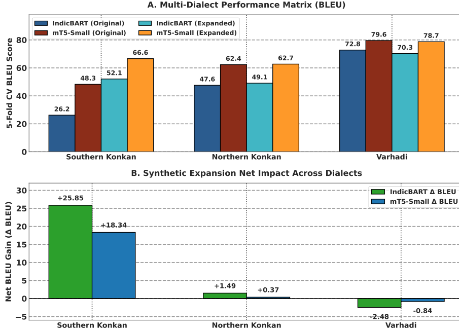
Fig. 6. Multi-dialect 5-fold cross-validation benchmark comparison: (A) Absolute BLEU scores across model architectures and corpora partitions, and (B) Net synthetic expansion impact ( \Delta BLEU across sub-dialects).
