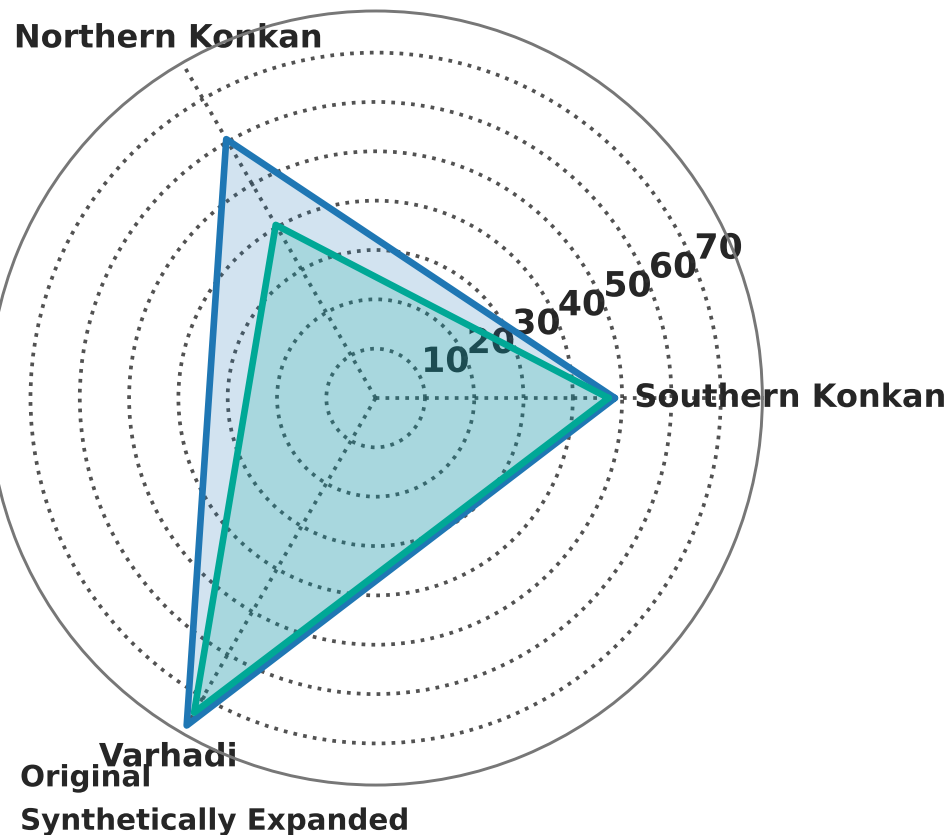
A. IndicBART Radar Profile
