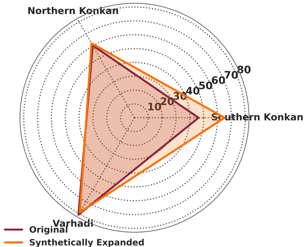
B. mT5-Small Radar Profile
