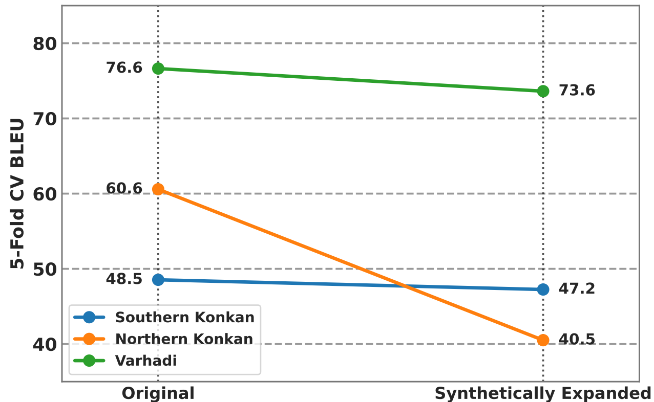
A. IndicBART (244M) Slope Chart
