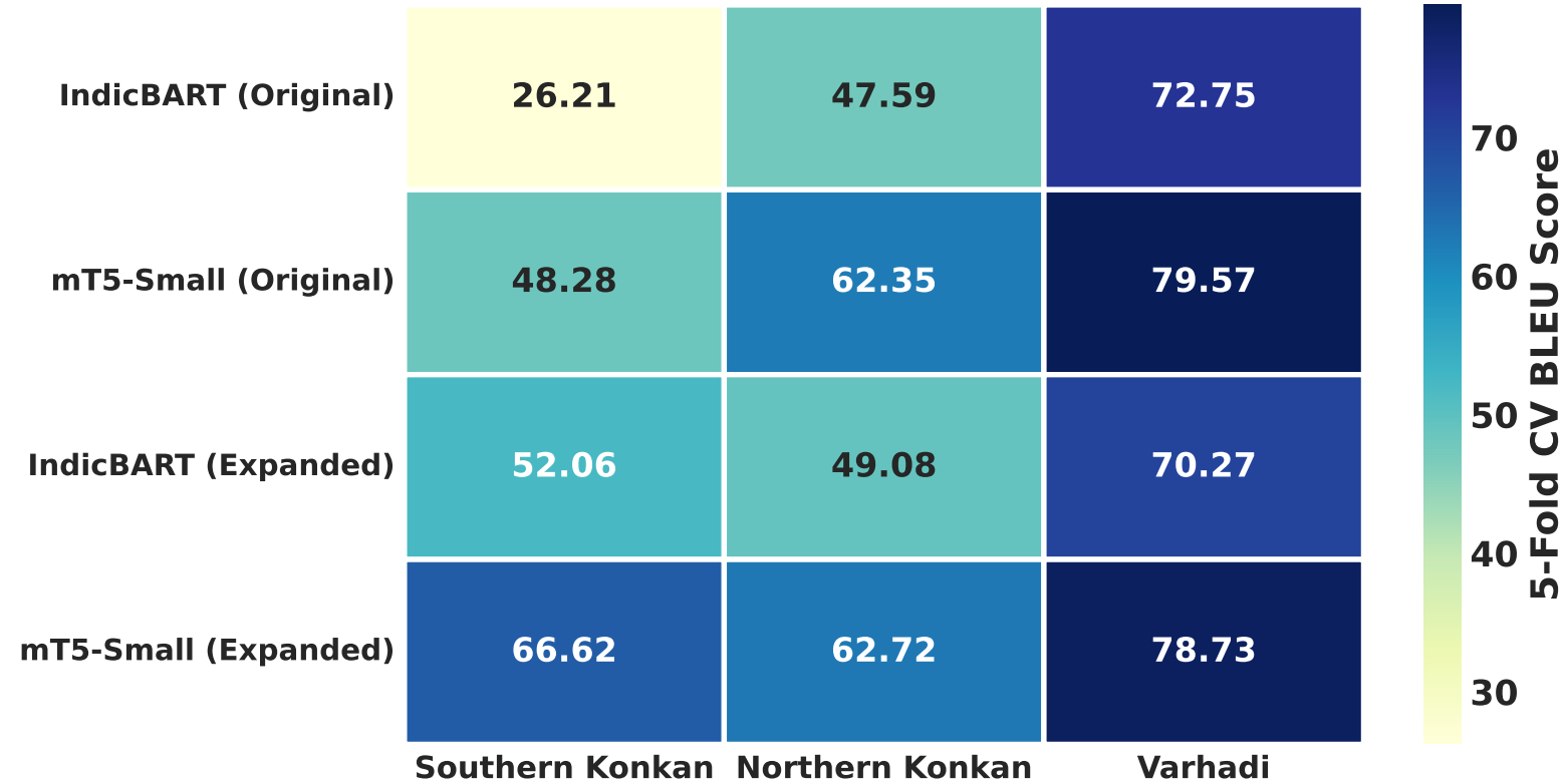
A. Multi-Dialect Performance Heatmap (BLEU)
