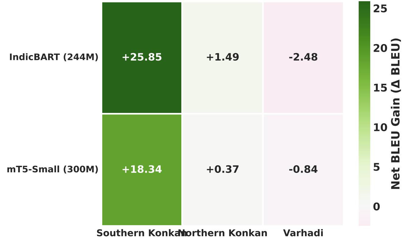
B. Synthetic Expansion Net Impact ( \Delta BLEU)
