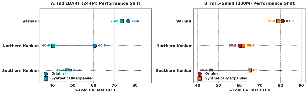
Figure 5: Single-dialect 5-fold cross-validation performance shift comparing Original and Synthetically Expanded models for IndicBART (244M) and mT5-small (300M).
