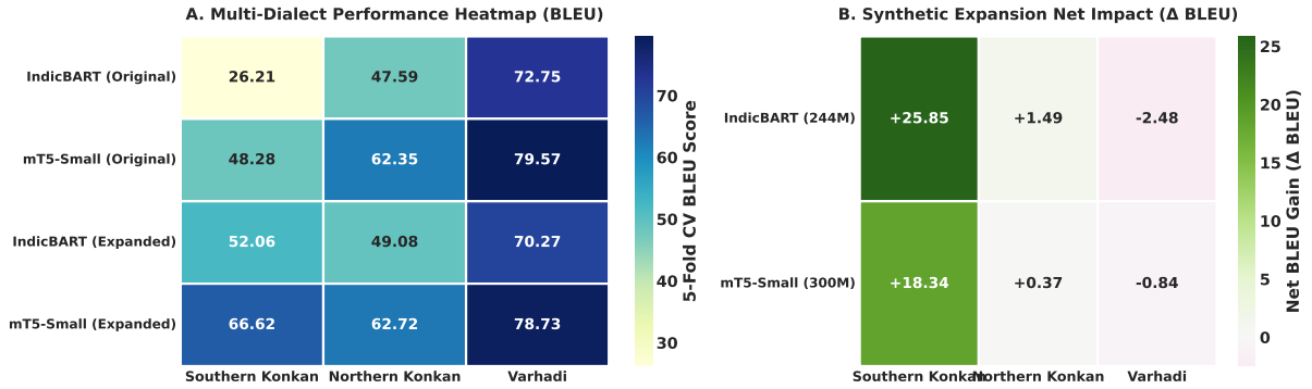
Figure 6: Multi-dialect 5-fold cross-validation performance matrix: (A) Absolute BLEU score heatmap across model architectures and corpora partitions, and (B) Net synthetic expansion impact ( \Delta BLEU).
