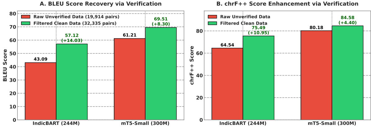
Figure 8: Multi-tier verification engine ablation: (A) BLEU score recovery and (B) chrF++ score enhancement comparing models trained on raw unverified synthetic outputs vs. filtered clean synthetic data.
