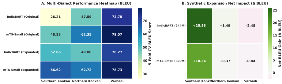
Fig. 6. Multi-dialect 5-fold cross-validation performance matrix: (A) Absolute BLEU score heatmap across model architectures and corpora partitions, and (B) Net synthetic expansion impact ( \Delta BLEU).
