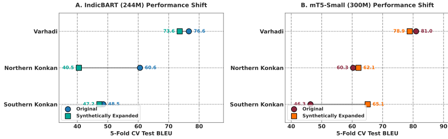
Fig. 5. Single-dialect 5-fold cross-validation performance shift comparing Original and Synthetically Expanded models for IndicBART (244M) and mT5-small (300M).
