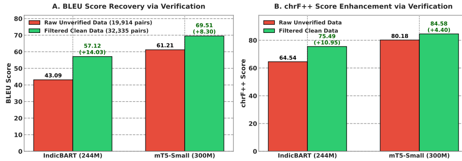
Fig. 8. Multi-tier verification engine ablation: (A) BLEU score recovery and (B) chrF++ score enhancement comparing models trained on raw unverified synthetic outputs vs. filtered clean synthetic data.
