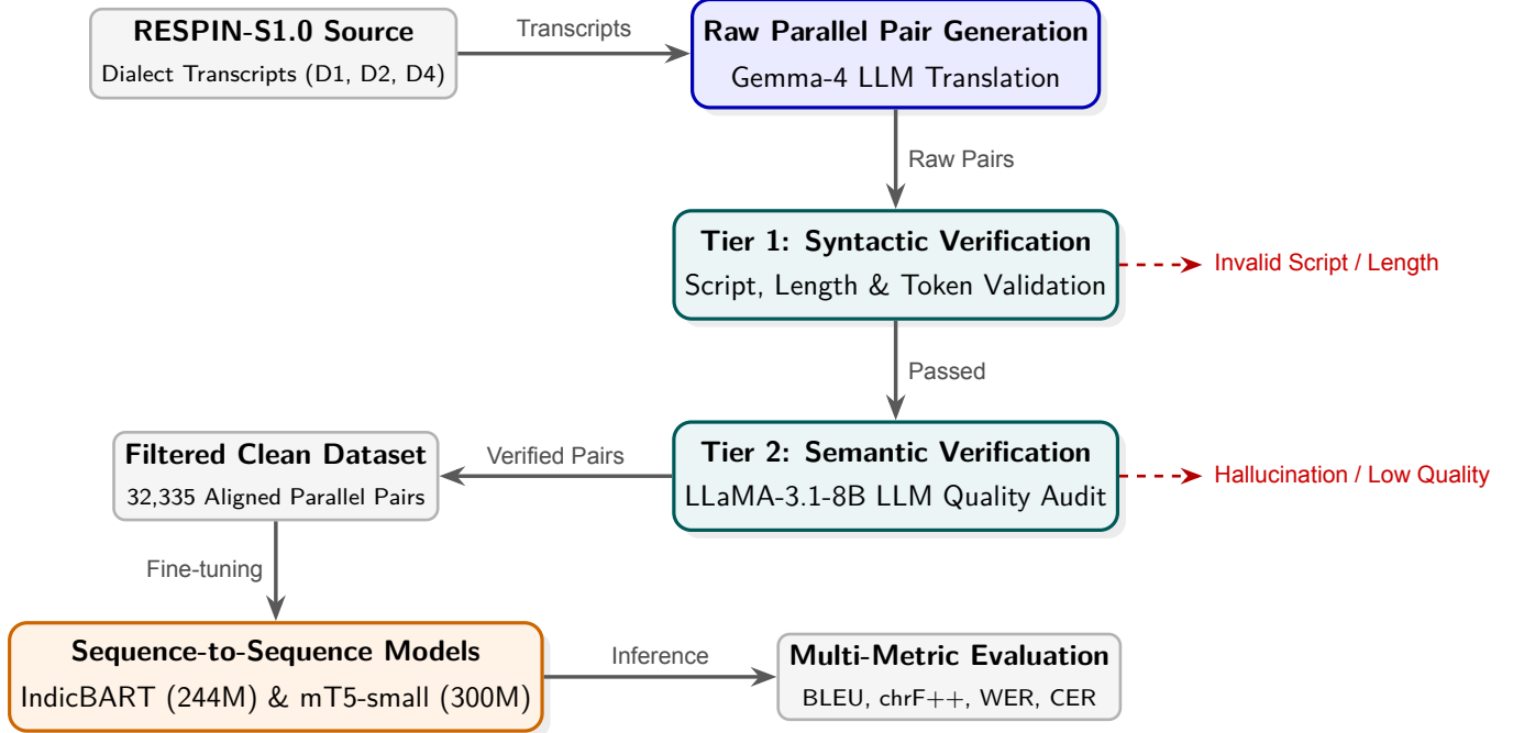
Figure 2: End-to-end multi-dialect Marathi text normalization framework: raw pair generation using Gemma-4, multi-tier syntactic/semantic verification, and conditioned sequence-to-sequence model fine-tuning.
