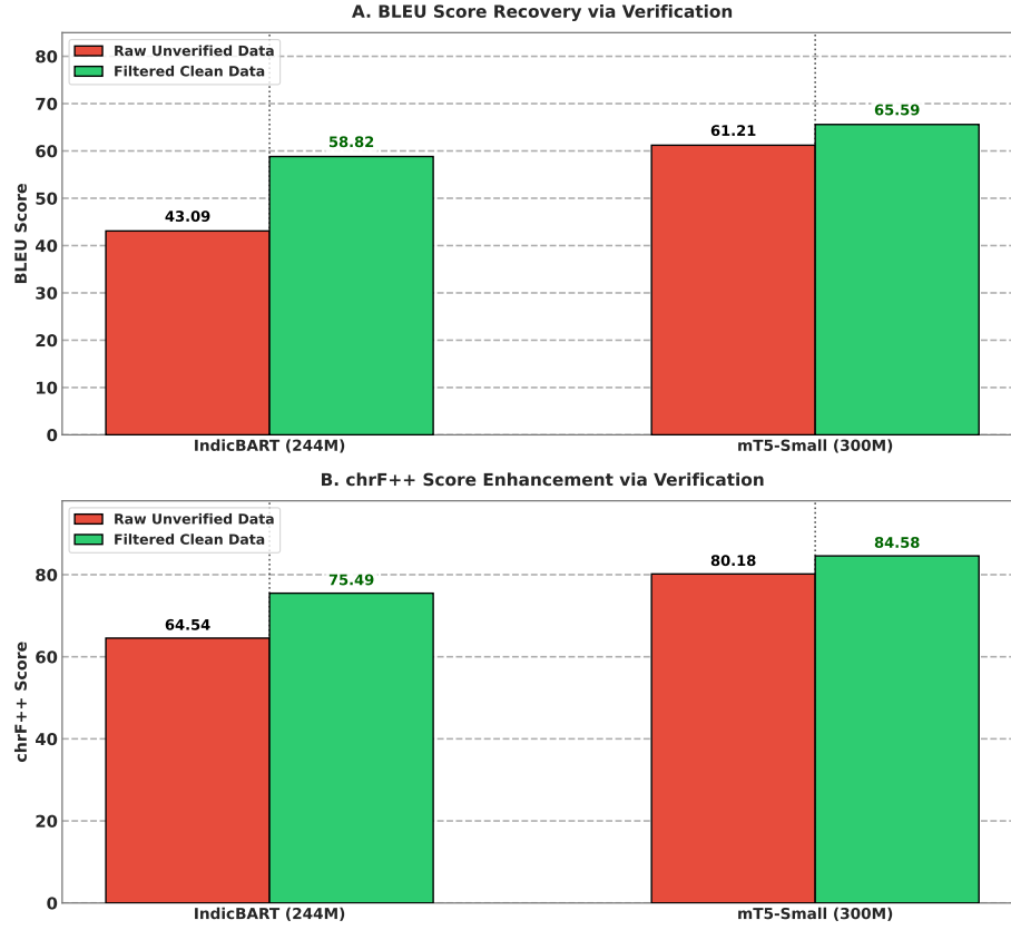
Fig.8. Multi-tier verification engine ablation: (A) BLEU score recovery and (B) chrF++ score enhancement comparing models trained on raw unverified synthetic outputs vs. filtered clean synthetic data.
