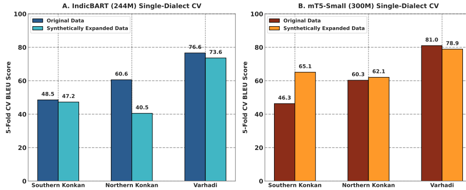
Fig. 5. Single-dialect 5-fold cross-validation performance shift comparing Original and Synthetically Expanded models for IndicBART (244M) and mT5-small (300M).
