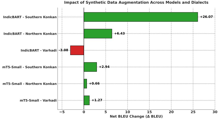
Fig. 7. Impact of LLM synthetic data expansion ( \Delta BLEU score comparing synthetically expanded vs. original benchmarks on the held-out test set).
