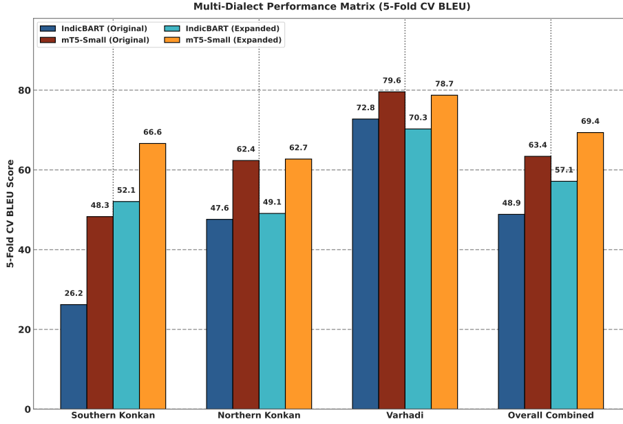
Fig. 6. Multi-dialect 5-fold cross-validation benchmark comparison: (A) Absolute BLEU scores across model architectures and corpora partitions, and (B) Net synthetic expansion impact ( \Delta BLEU across sub-dialects).
