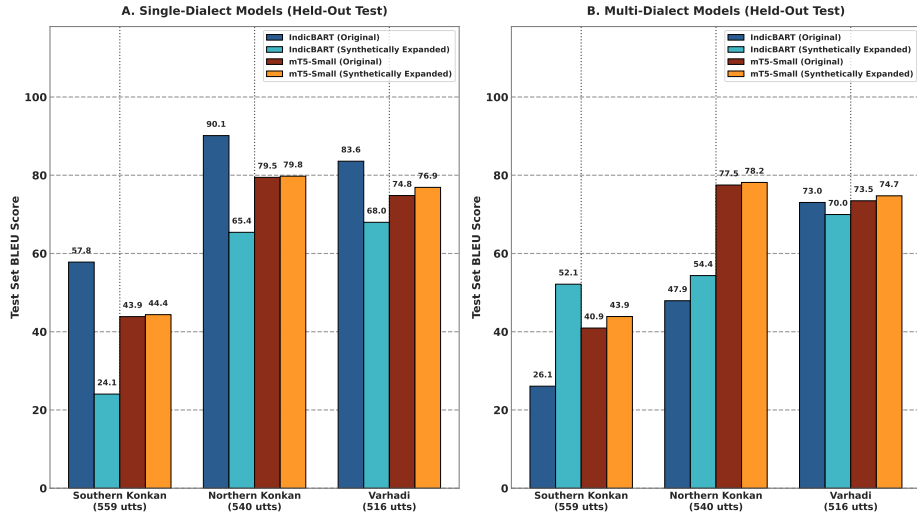
Fig. 4. Comprehensive sequence-to-sequence evaluation matrix on the held-out RESPIN test benchmark (2,170 utterances), comparing IndicBART (244M) and mT5-small (300M) across single-dialect and multi-dialect training configurations.
