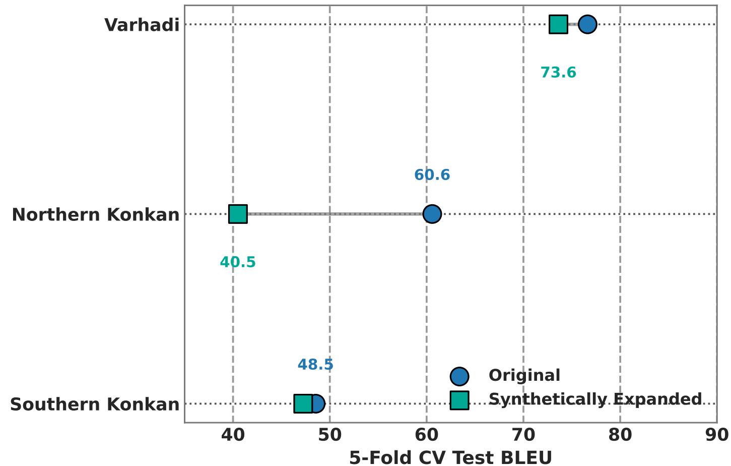
A. IndicBART (244M) Single-Dialect Performance Shift
