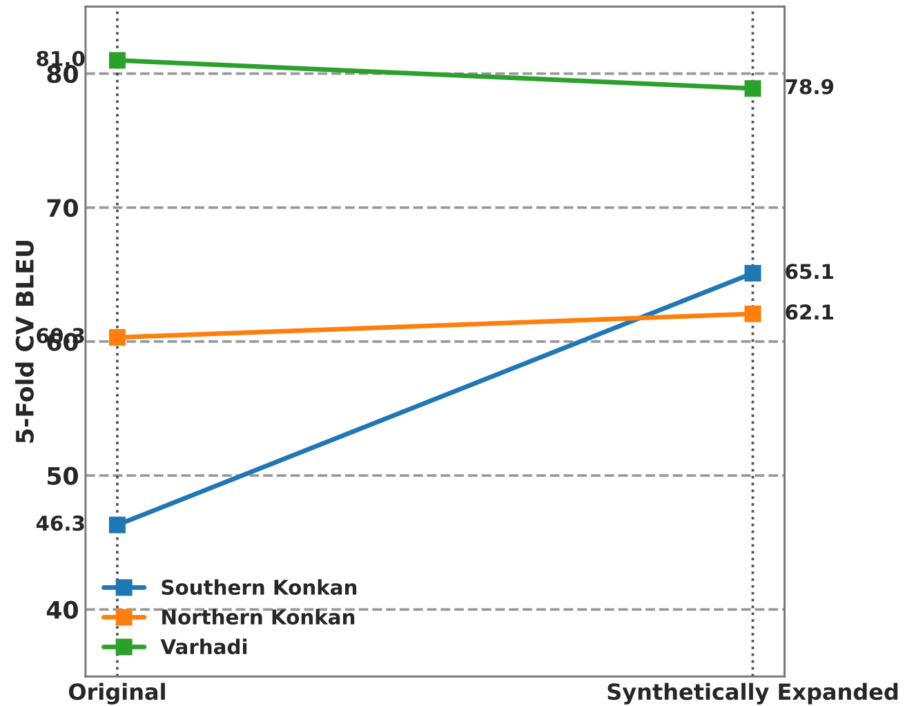
B. mT5-Small (300M) Slope Chart
