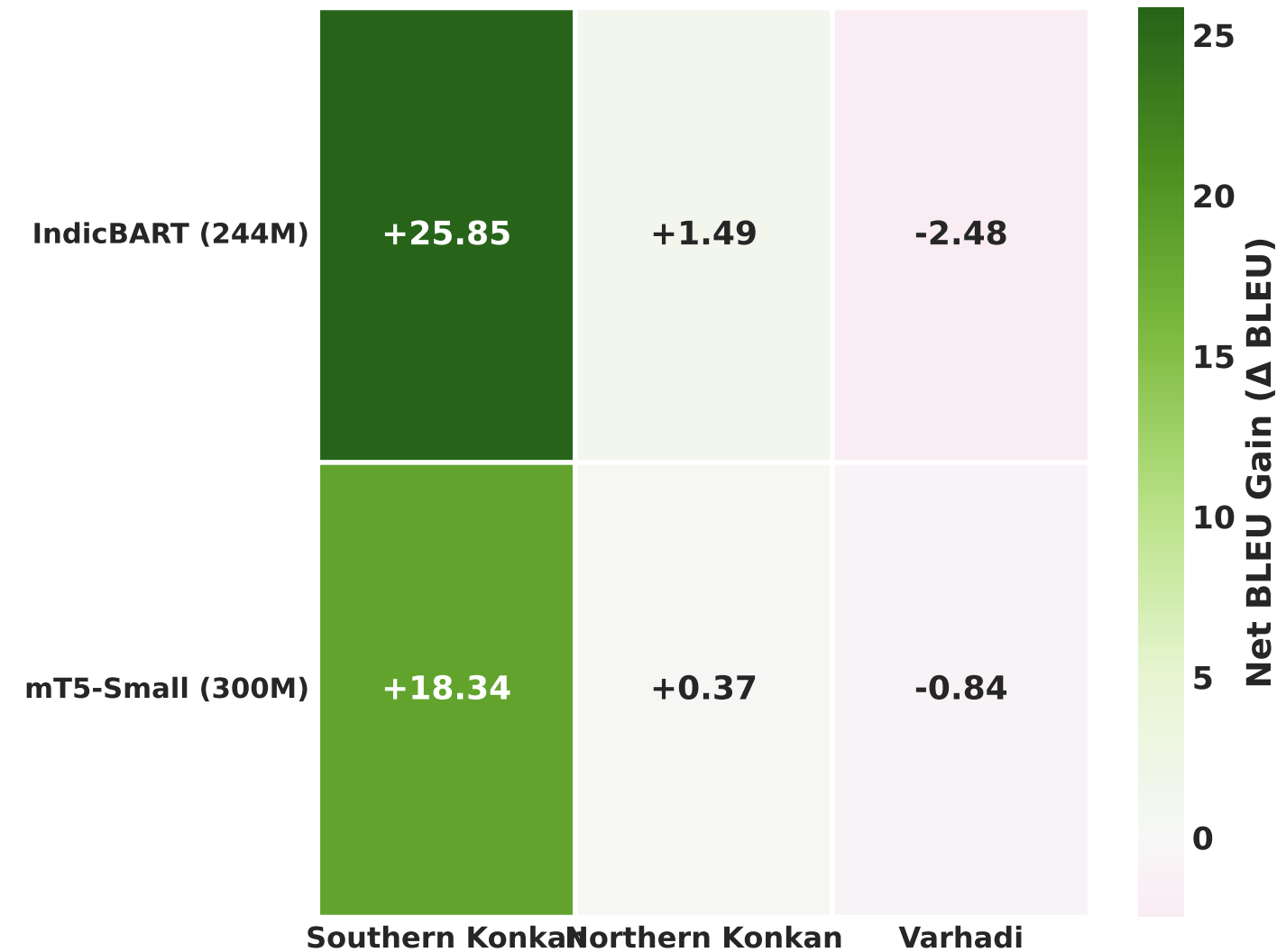
B. Synthetic Expansion Net Impact ( \Delta BLEU)
