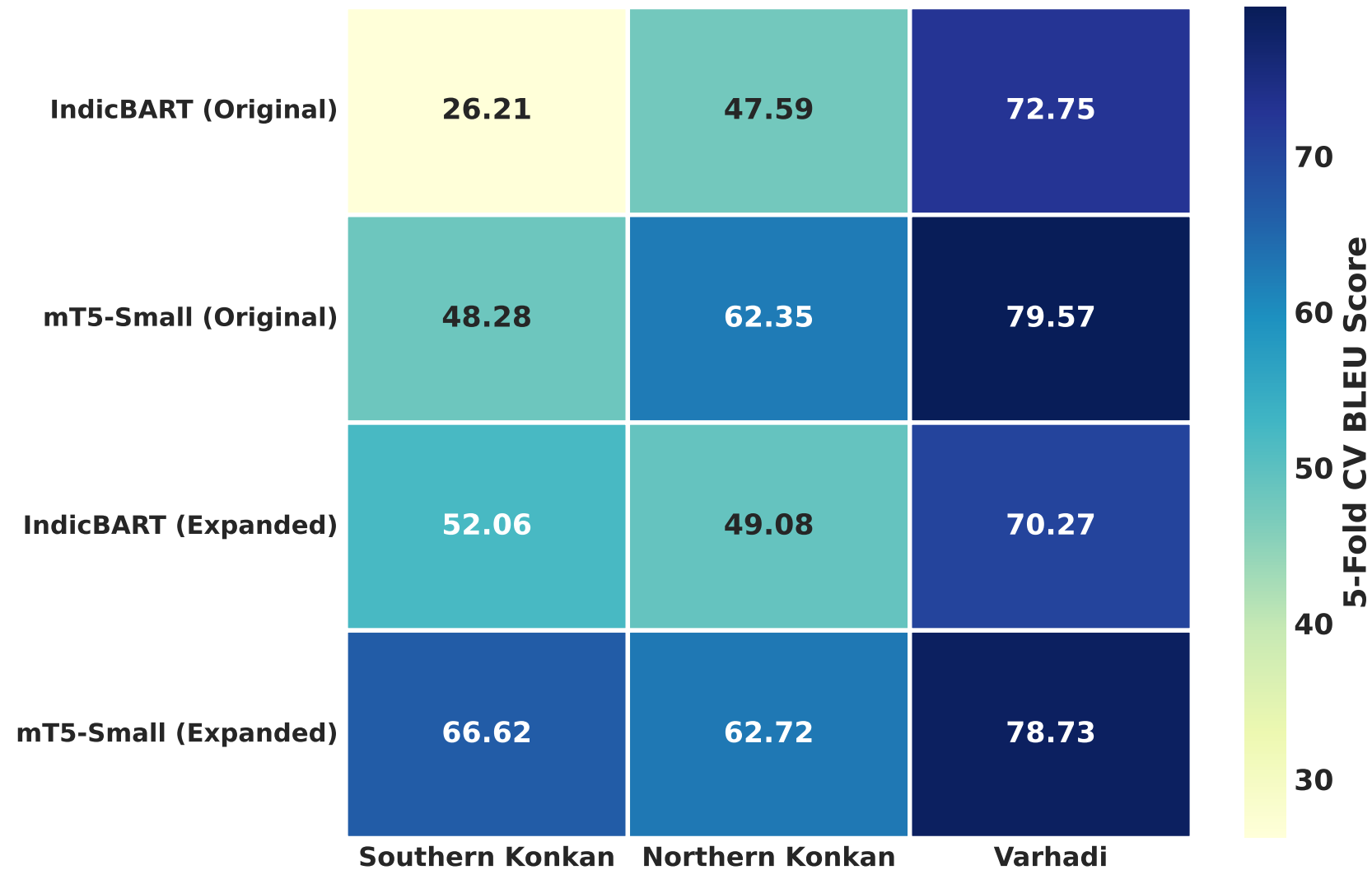
A. Multi-Dialect Performance Heatmap (BLEU)
