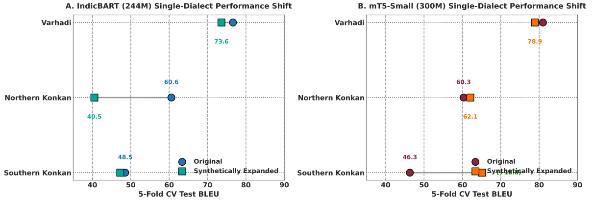
Figure 5: Single-dialect 5-fold cross-validation performance shift (Dumbbell Plot) comparing Original and Synthetically Expanded models for IndicBART (244M) and mT5-small (300M).
