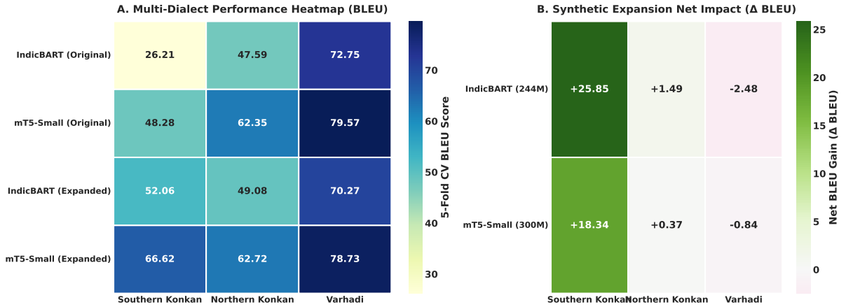
Figure 8: Multi-dialect 5-fold cross-validation performance matrix: (A) Absolute BLEU score heatmap across model architectures and corpora partitions, and (B) Net synthetic expansion impact ( \Delta BLEU).
