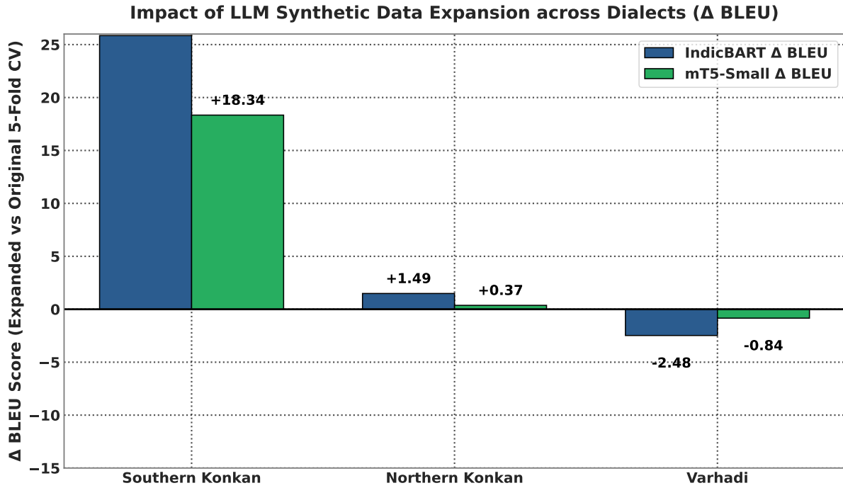
Figure 9: Impact of LLM synthetic data expansion ( \Delta BLEU score comparing synthetically expanded vs. original 5-fold cross-validation benchmarks).
