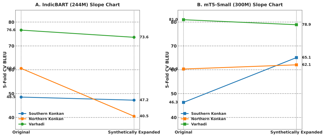
Figure 6: Single-dialect 5-fold cross-validation slope chart tracking BLEU score trajectories from Original to Synthetically Expanded corpora.
