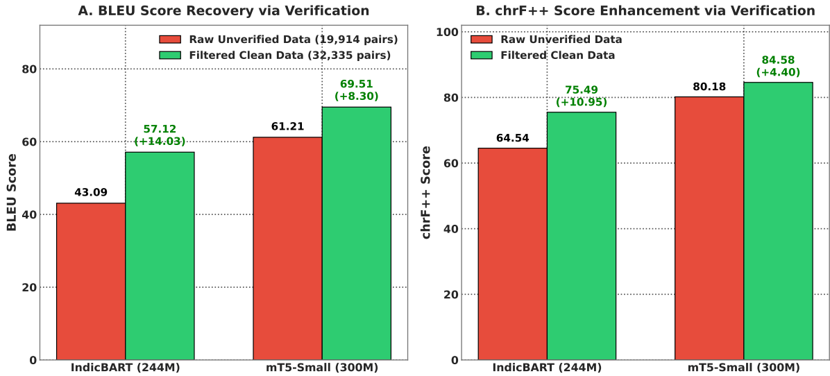
Figure 10: Multi-tier verification engine ablation: (A) BLEU score recovery and (B) chrF++ score enhancement comparing models trained on raw unverified synthetic outputs vs. filtered clean synthetic data.
