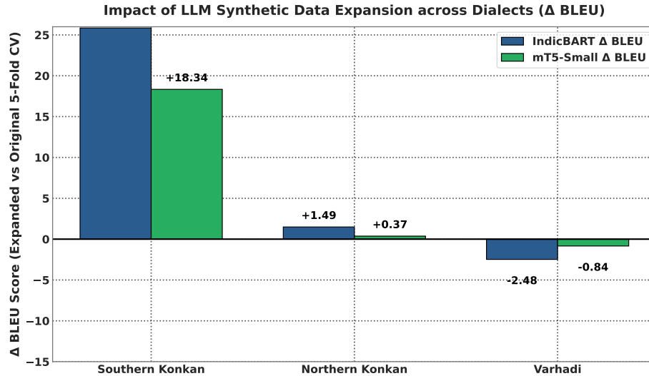
Fig. 9. Impact of LLM synthetic data expansion ( \Delta BLEU score comparing synthetically expanded vs. original 5-fold cross-validation benchmarks).
