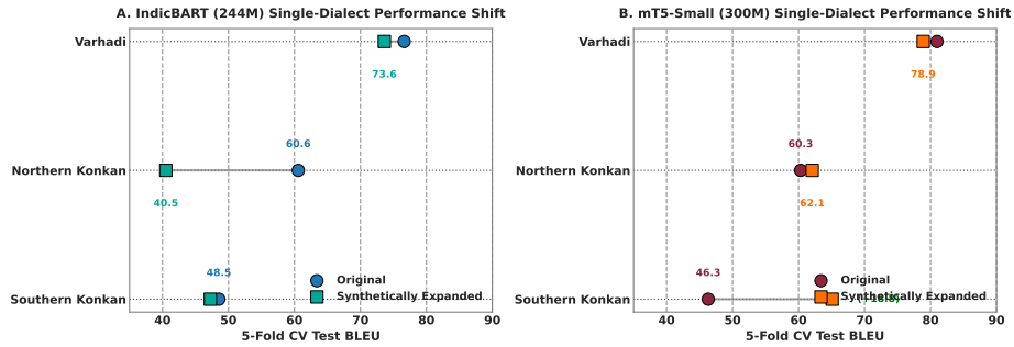
Fig. 5. Single-dialect 5-fold cross-validation performance shift (Dumbbell Plot) comparing Original and Synthetically Expanded models for IndicBART (244M) and mT5-small (300M).
