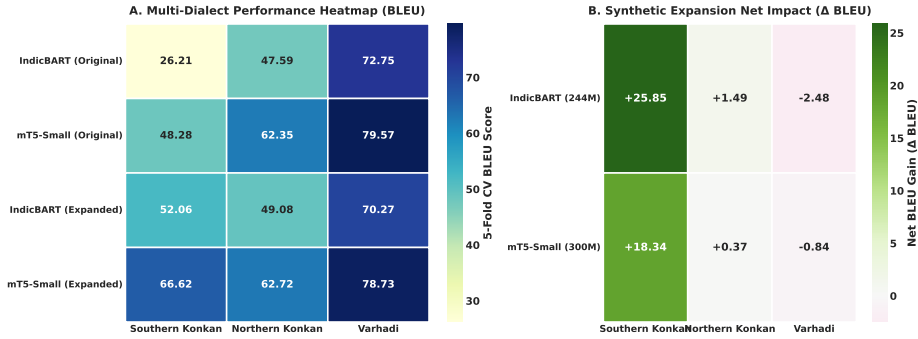
Fig. 8. Multi-dialect 5-fold cross-validation performance matrix: (A) Absolute BLEU score heatmap across model architectures and corpora partitions, and (B) Net synthetic expansion impact ( \Delta BLEU).
