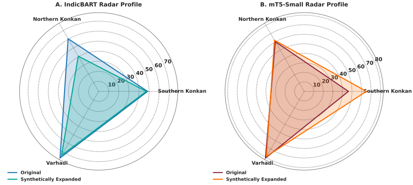
Fig. 7. Single-dialect polar radar profile comparison illustrating benchmark metric coverage across sub-dialects for IndicBART (244M) and mT5-small (300M).
