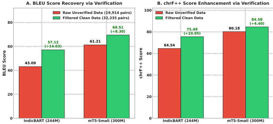
Fig. 10. Multi-tier verification engine ablation: (A) BLEU score recovery and (B) chrF++ score enhancement comparing models trained on raw unverified synthetic outputs vs. filtered clean synthetic data.
