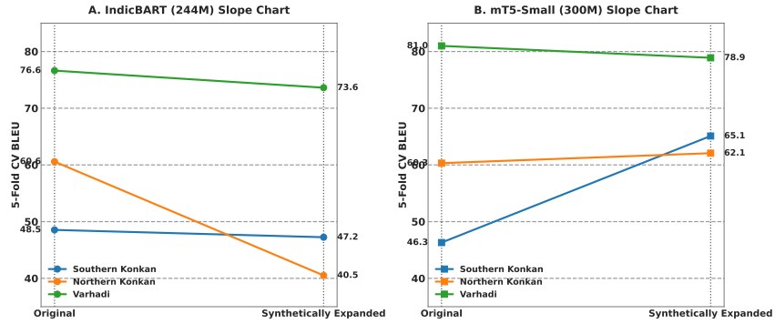
Fig. 6. Single-dialect 5-fold cross-validation slope chart tracking BLEU score trajectories from Original to Synthetically Expanded corpora.
