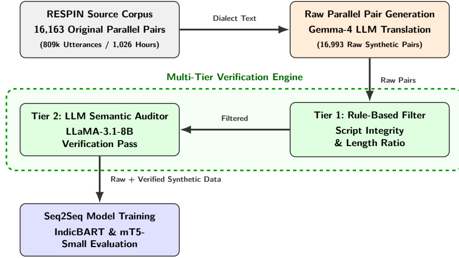
Fig. 2. System architecture of the given multi-dialect normalization framework.
