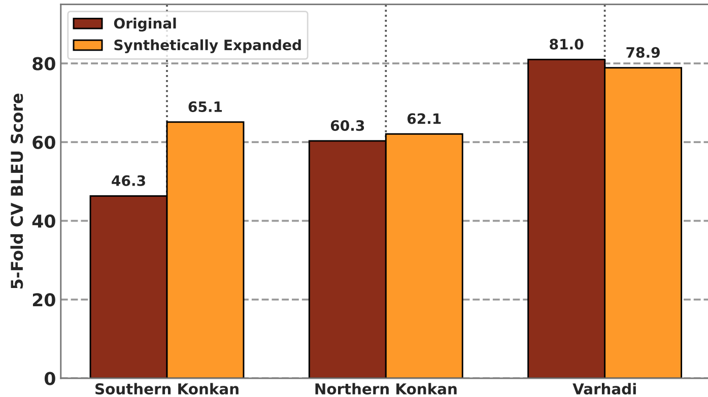
B. mT5-Small (300M) Single-Dialect CV BLEU
