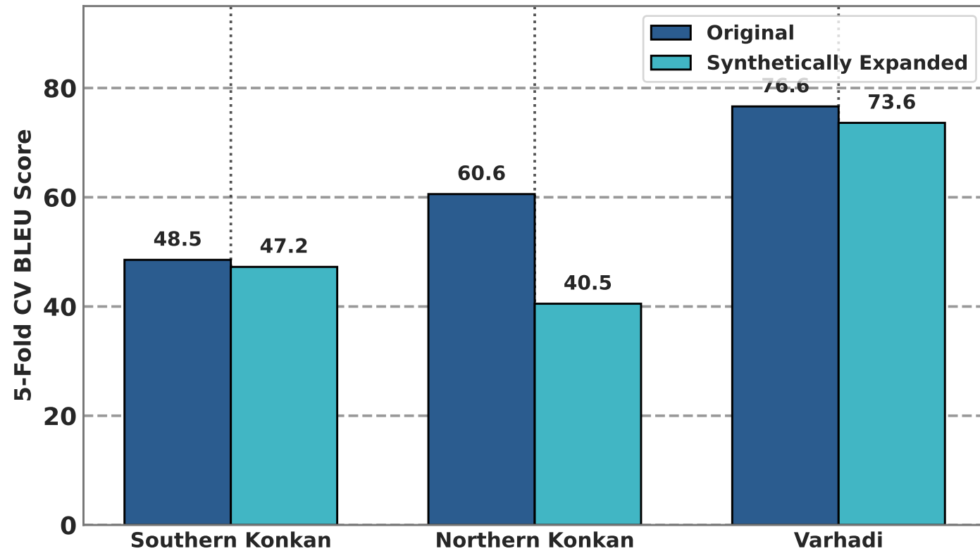
A. IndicBART (244M) Single-Dialect CV BLEU
