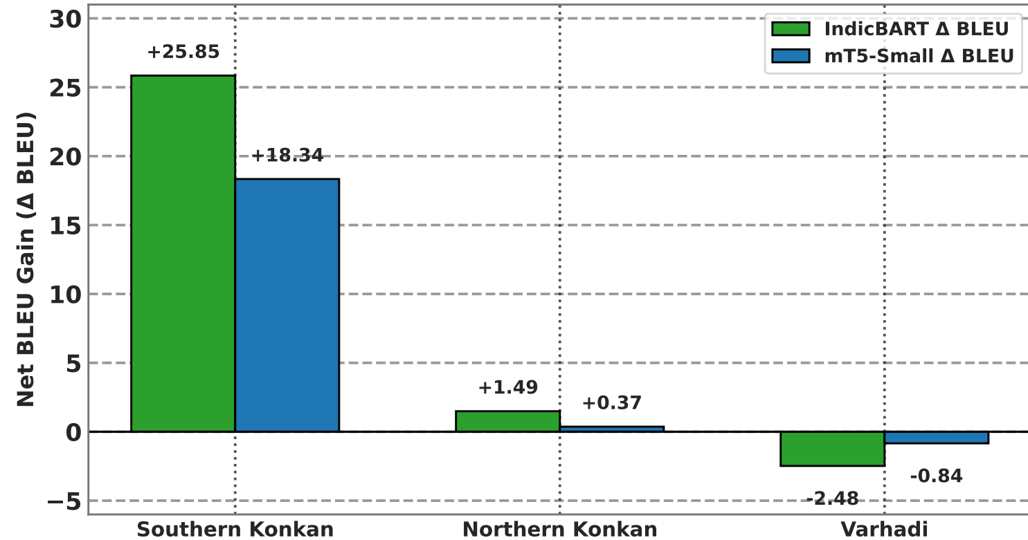
B. Synthetic Expansion Net Impact Across Dialects
