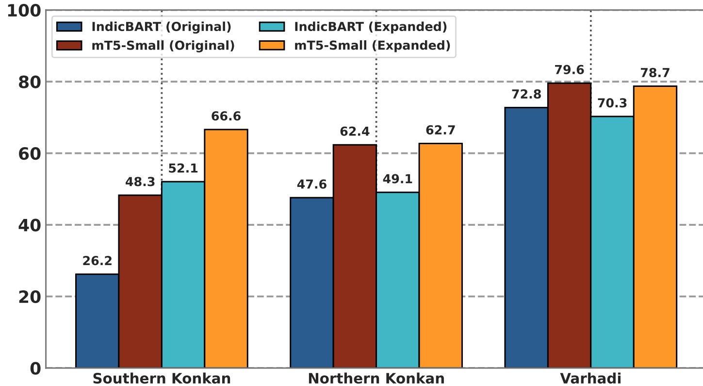
A. Multi-Dialect Performance Matrix (BLEU)
