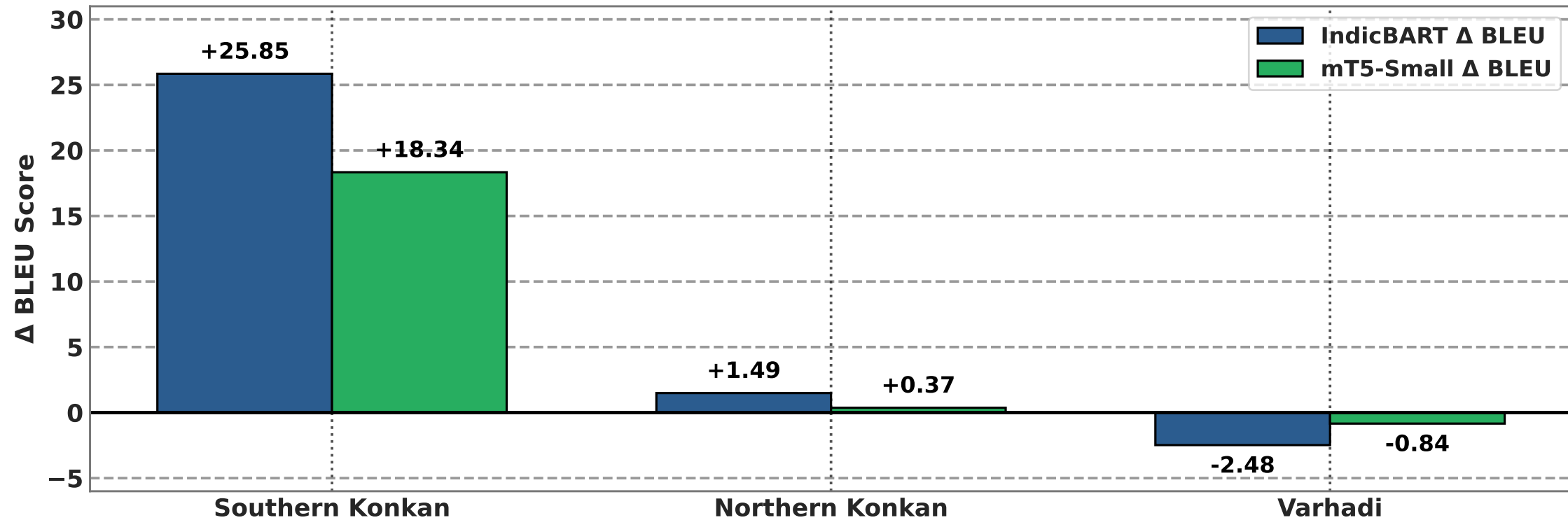
Impact of LLM Synthetic Data Expansion across Dialects ( \Delta BLEU)
