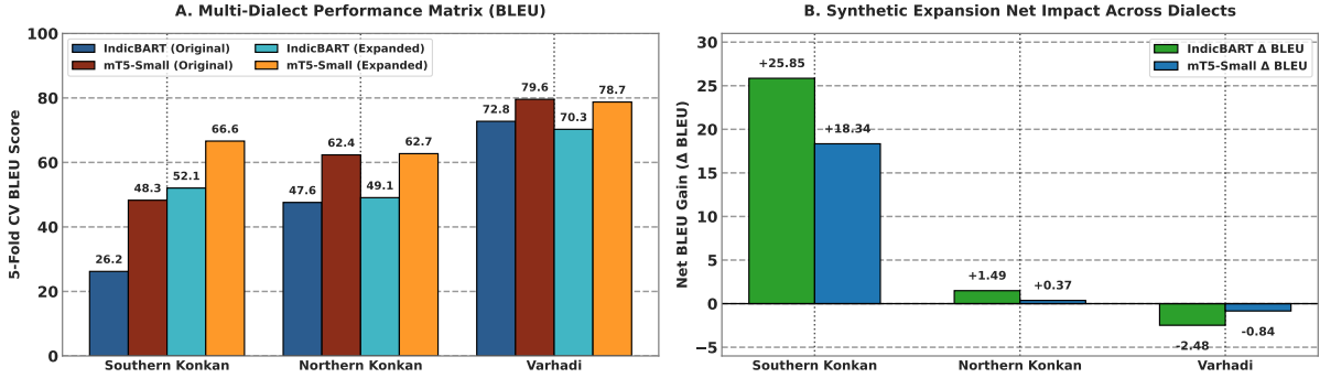
Figure 6: Multi-dialect 5-fold cross-validation benchmark comparison: (A) Absolute BLEU scores across model architectures and corpora partitions, and (B) Net synthetic expansion impact ( \Delta BLEU across sub-dialects).
