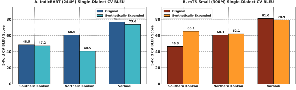
Figure 5: Single-dialect 5-fold cross-validation performance shift comparing Original and Synthetically Expanded models for IndicBART (244M) and mT5-small (300M).
