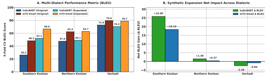
Fig. 6. Multi-dialect 5-fold cross-validation benchmark comparison: (A) Absolute BLEU scores across model architectures and corpora partitions, and (B) Net synthetic expansion impact ( \Delta BLEU across sub-dialects).
