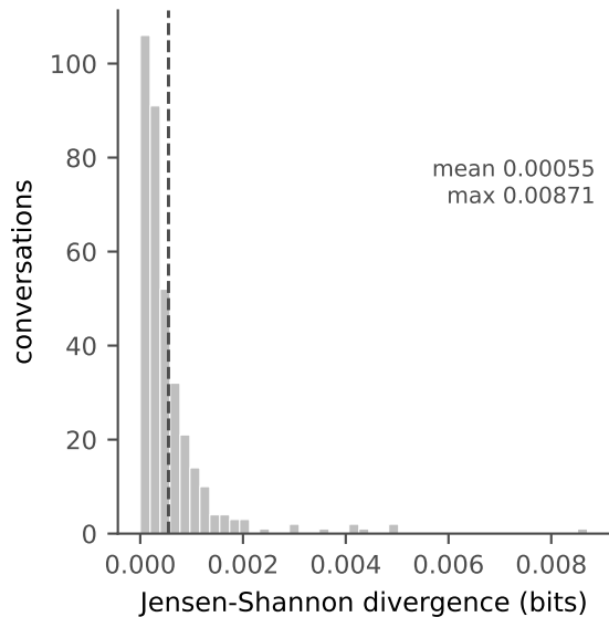
JSD, secondary (see fig2c for why)
