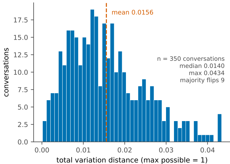
Label shift from the published filter TVD, primary metric
