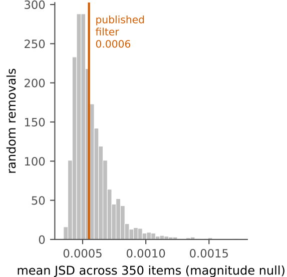
Published filter vs removing 19 raters at random (2000 draws)
