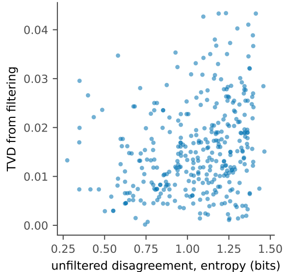
Shift vs disagreement Spearman \rho = +0.266 (n=350)
