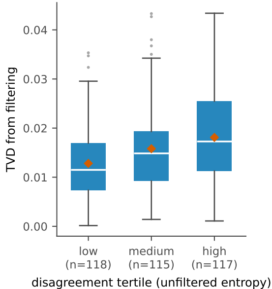
Filtering effect by how contested the item is
