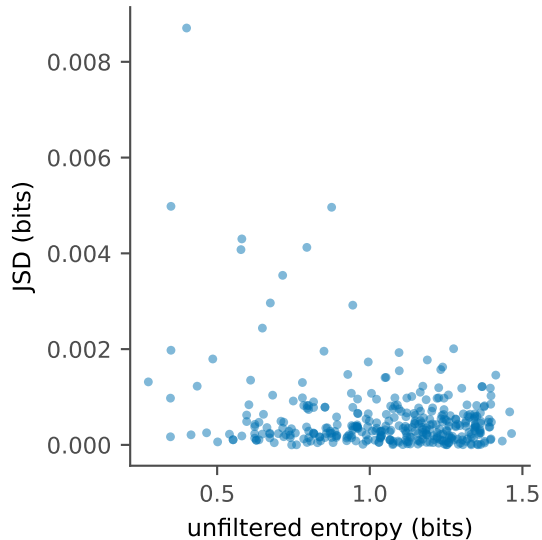
JSD vs disagreement low-entropy outliers dominate
