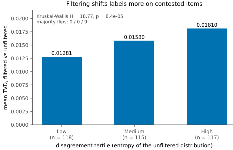
Figure 2: Mean TVD between filtered and unfiltered item distributions by disagreement tertile ( n = 118, 115, 117 ). The increase is monotonic, Kruskal-Wallis p = 8.4\text{e-}05 , and is consistent with the tie-aware majority-flip pattern of 0, 0 and 9.
