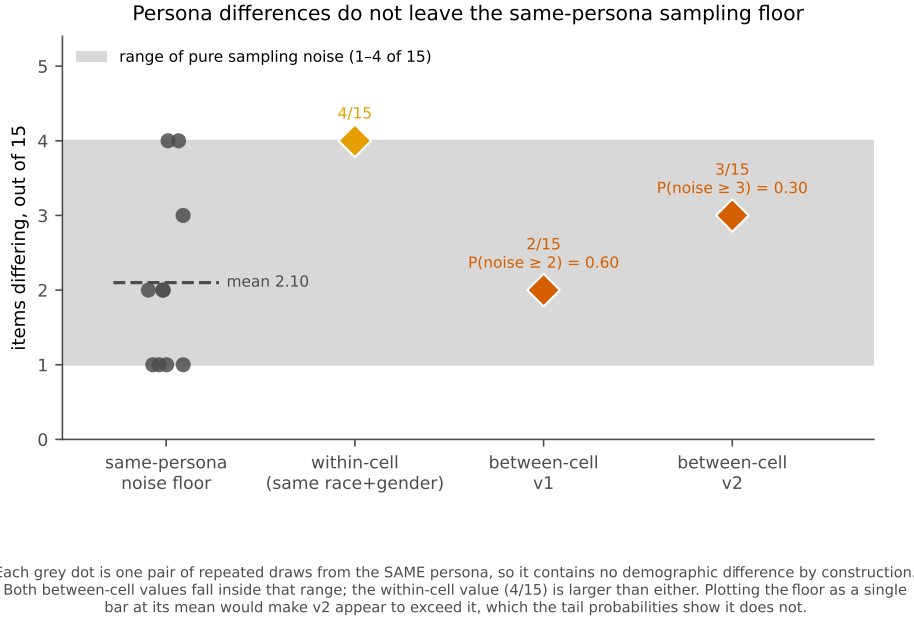
Figure 3: Persona differences against the same-persona sampling floor. Each grey point is one pair of repeated draws from the same persona and therefore contains no demographic difference by construction; the shaded band is their full range (1–4 of 15). Both between-cell values fall inside that band, with P(\text{noise} \geq \text{observed}) of 0.60 for v1 and 0.30 for v2. The within-cell comparison (4/15) is larger than either between-cell value.
