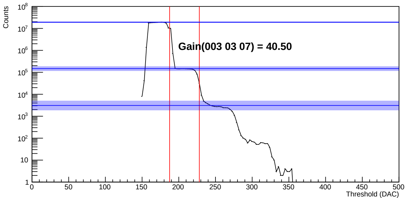
Threshold Scan Scaler Count Rates
