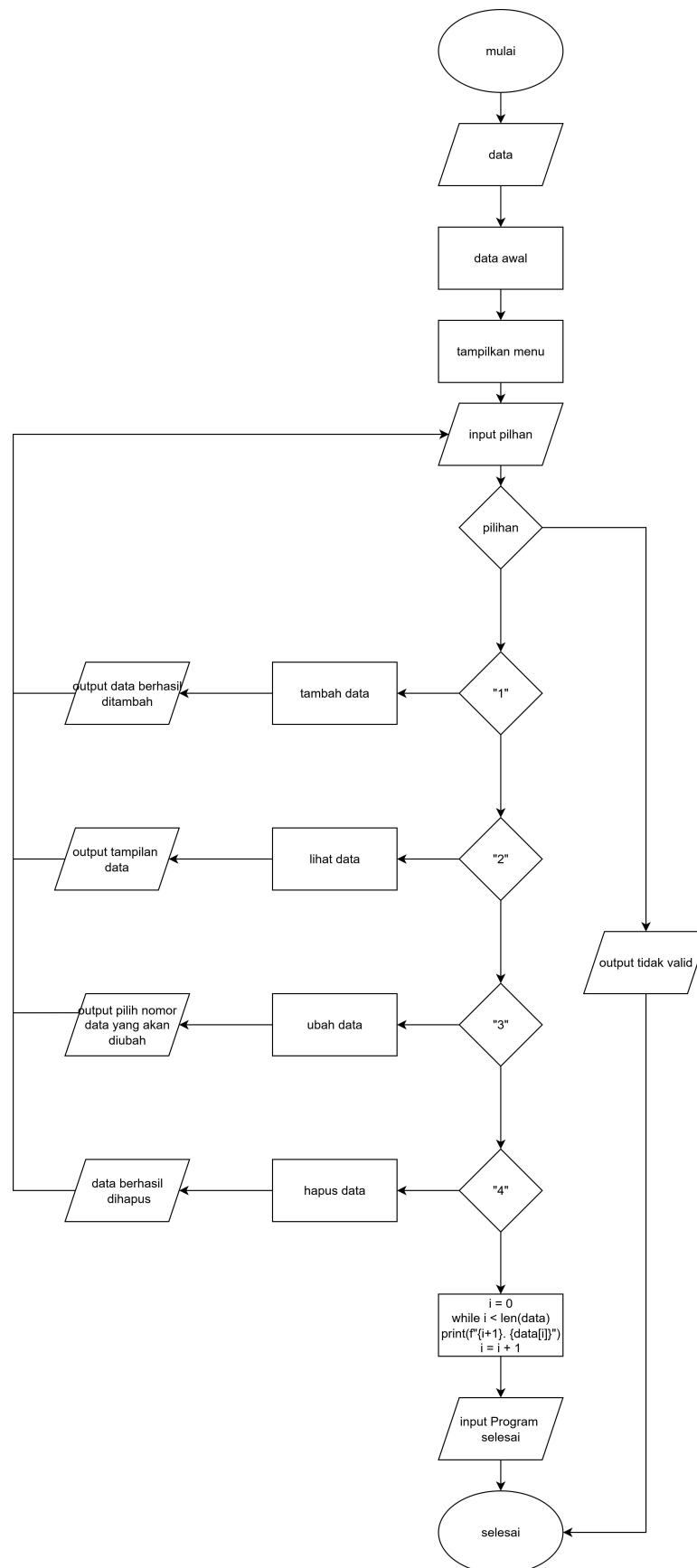
Gambar 1.1 Flowchart
