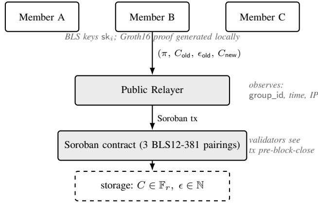
Figure 1. Onym data and metadata flow. Each member holds a BLS12-381 secret key and produces a 192-byte Groth16 proof \pi locally; one member submits the update tuple via a public relayer that pays the transaction fee. The Soroban contract verifies the proof using three BLS12-381 pairings and writes the new 32-byte commitment C_{\text{new}} and incremented epoch to storage. Italicized callouts mark the metadata each non-member party in the path observes.
