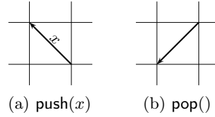
Figure 2.26: Stack updates
