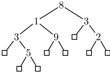
Extended binary tree
