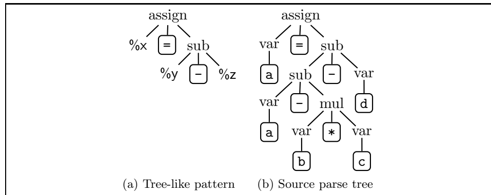
Figure 4: Tree pattern matching a = a - b*c - d
