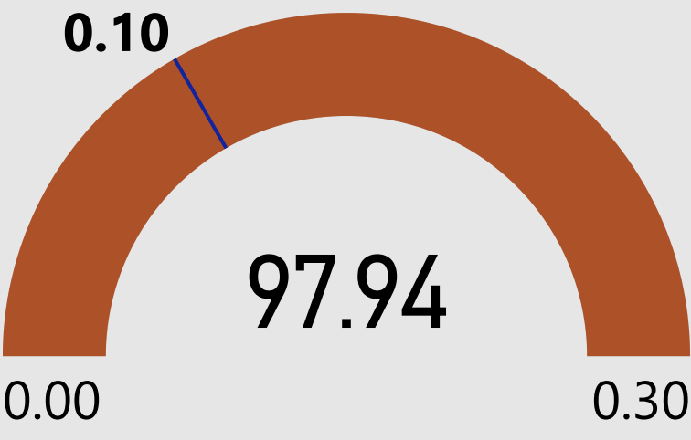
MAPE (Daily)
