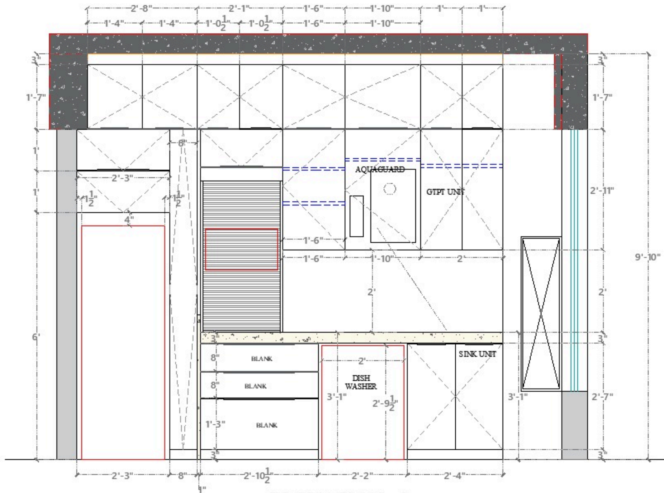
ELEVATION -C
