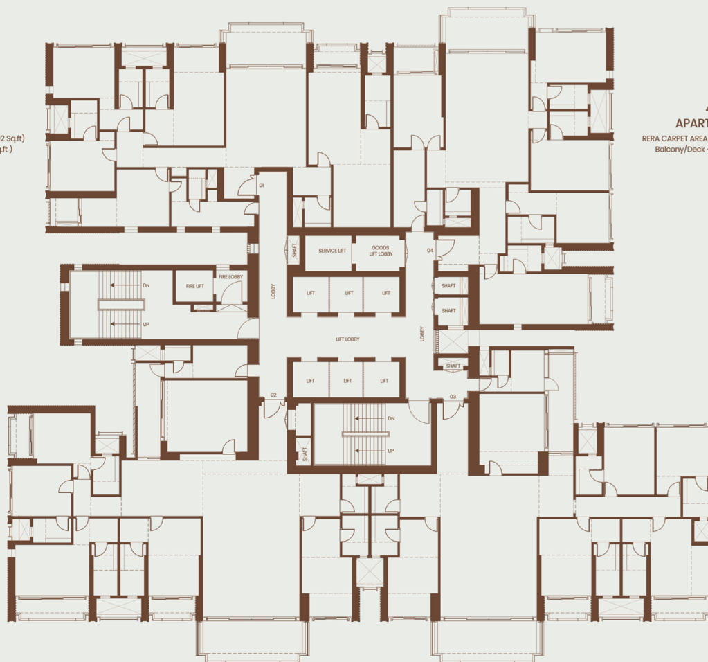
5 BHK APARTMENT-02 RERA CARPET AREA - 361.09 Sq.m(3887 Sq.ft) Balcony/Deck - 37.18 Sq.m ( 400 Sq.ft )
