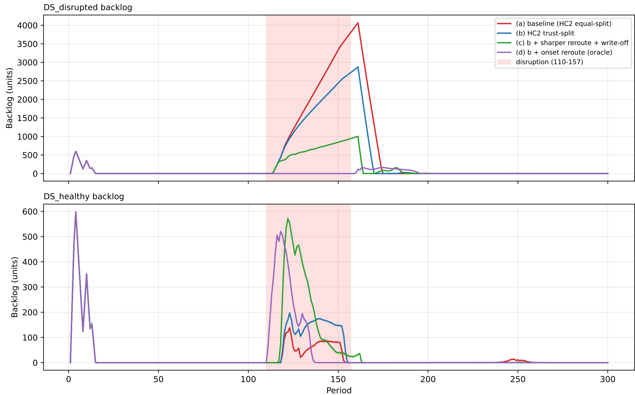
Routing ladder: distributor backlogs (urgent0, mean +/- SE, reporting seeds)
