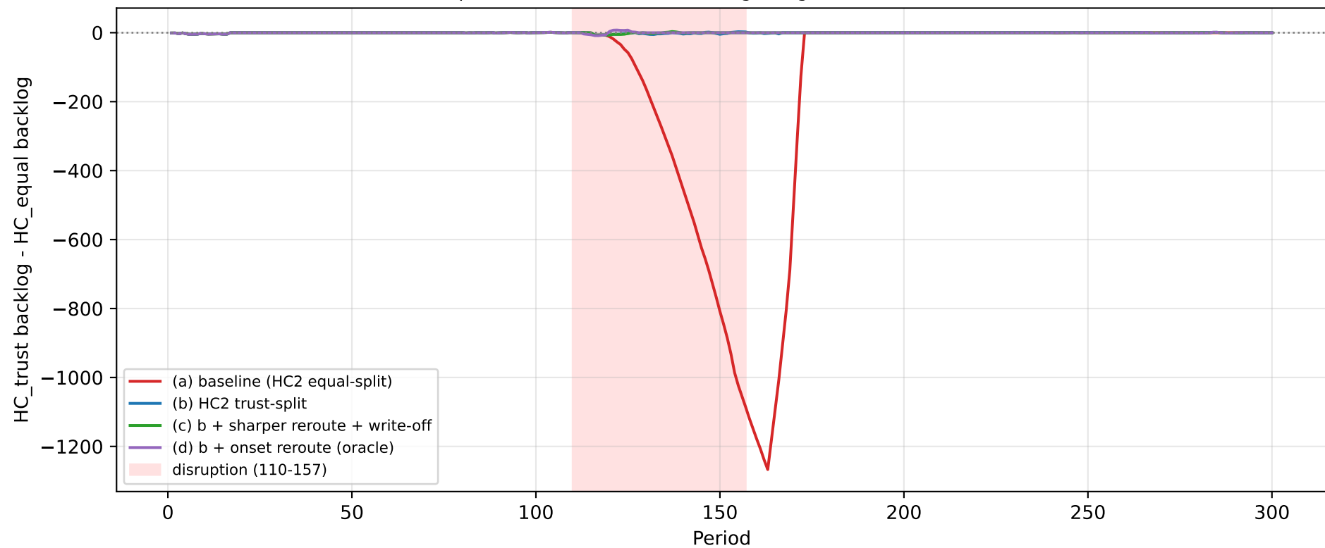
HC dispersion: who bears the shortage (urgent20, mean over seeds)
