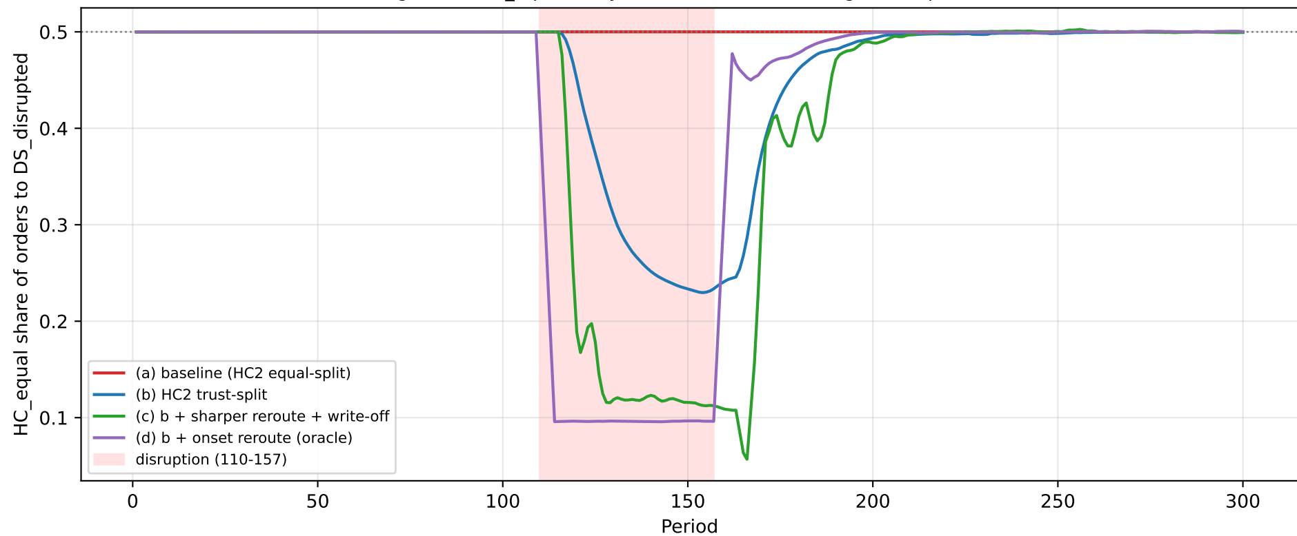
How fast each rung routes HC_equal away from the dead chain (urgent0, 5-period smoothed mean)
