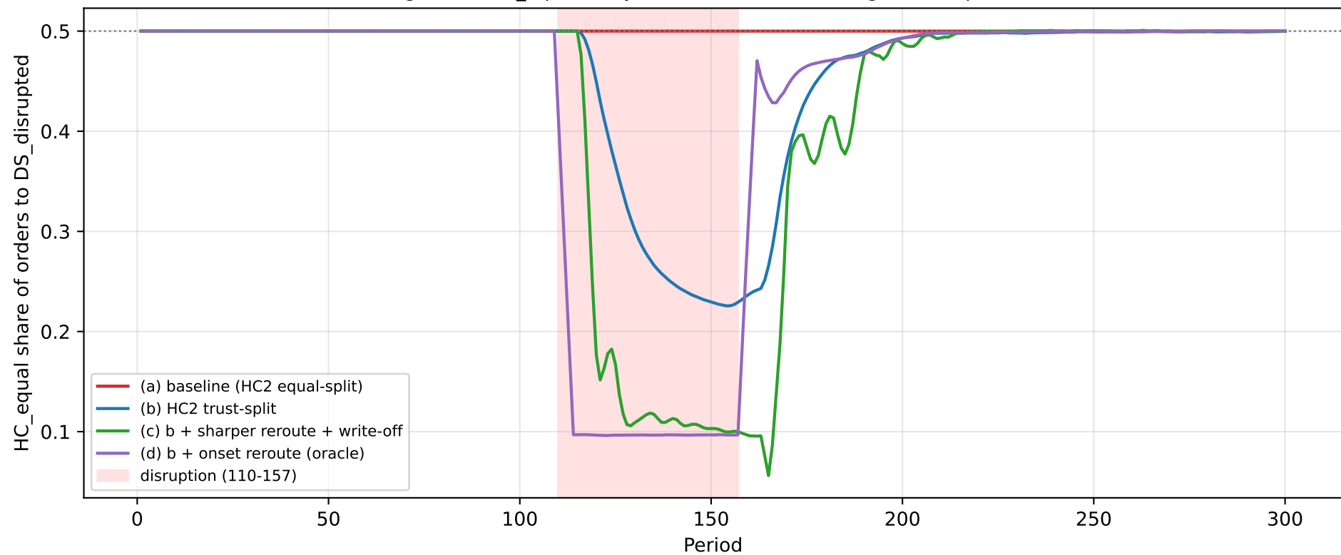
How fast each rung routes HC_equal away from the dead chain (urgent20, 5-period smoothed mean)
