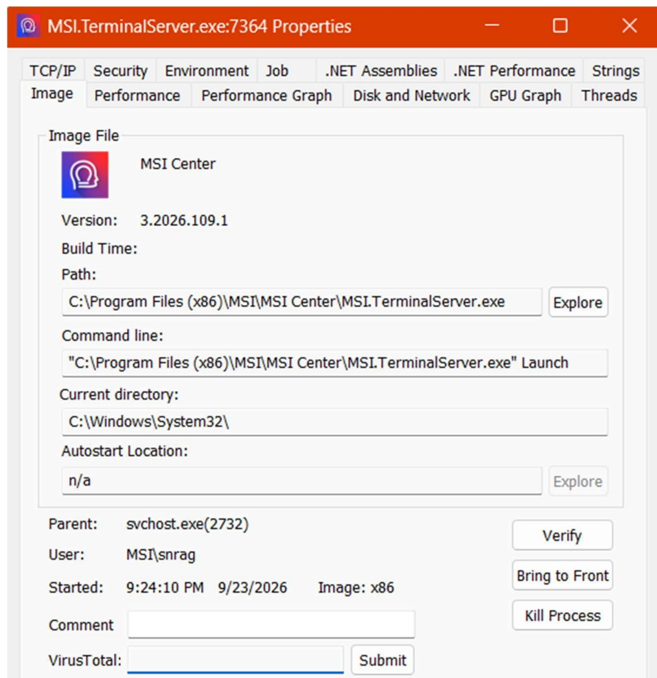
Figure 3: Inspecting image properties, cryptographic signatures, and execution file paths
