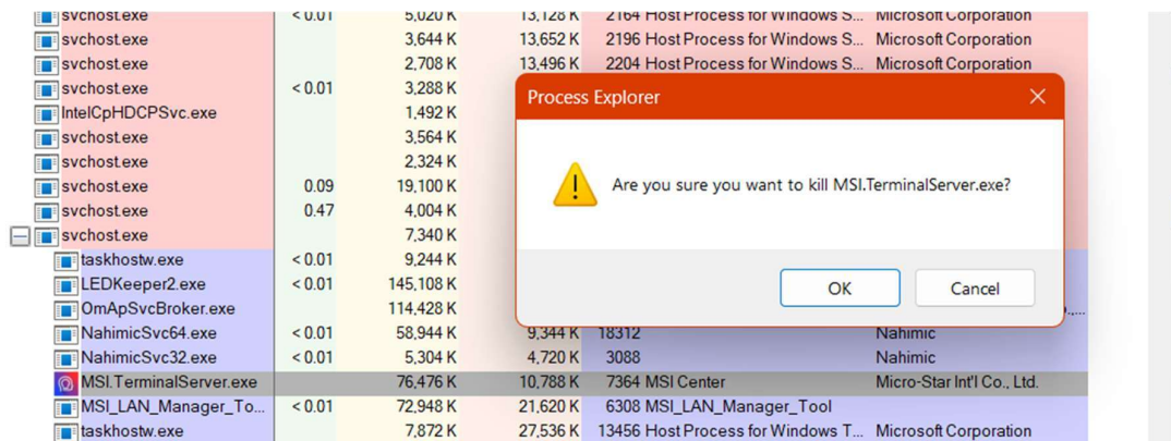
Figure 5: Terminating and suspending malicious process handles
