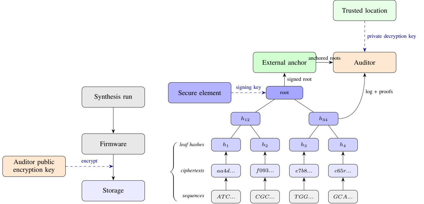
Figure 2. Log construction and verification. Each sequence is encrypted under the auditor’s public key; hashes of the resulting log entries form the leaves of a Merkle tree whose root is signed by the secure element and published to an external anchor. An auditor verifies integrity against anchored roots and recovers sequence content using the private decryption key held at a trusted location. Routine integrity verification re-hashes stored ciphertext and never requires decryption.
