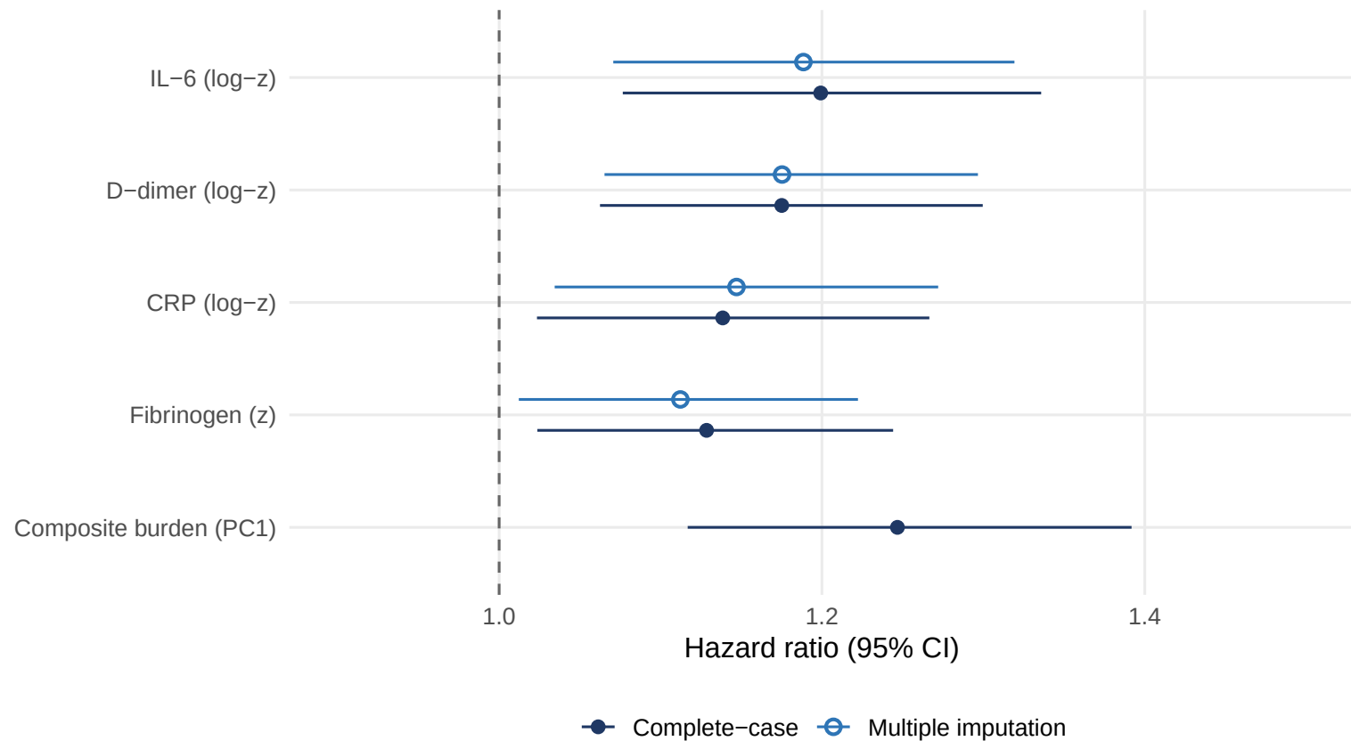
Figure 2. Adjusted hazard ratios for incident HF per 1-SD biomarker
