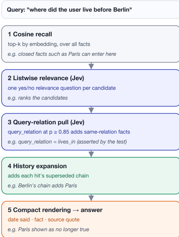
Figure 2: The read path on “where did the user live before Berlin” (fixture in
