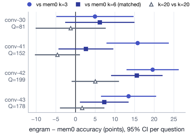
Figure 6: engram minus mem0 accuracy per held-out conversation, with per-question 95% intervals: engram k=3
