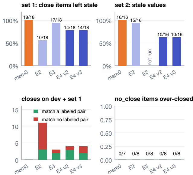
Figure 8: Store outcomes on the update sets: set-1 close items left stale, set-2 stale values, closes on
