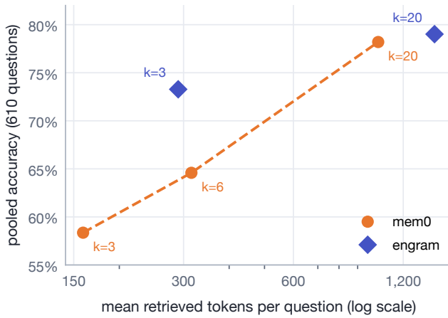
Figure 5: Pooled held-out accuracy (610 questions) against mean retrieved tokens per question. mem0
