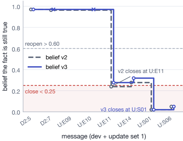
Figure 3: Belief in the fact “Melanie carves out daily me-time through running, reading, or playing violin”
