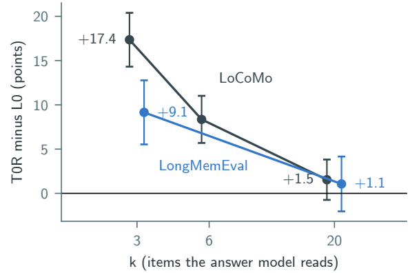
Figure 5: The rerank’s gain over similarity search (T0R minus L0, paired, in points, with 95% intervals) against k . LoCoMo: 778 questions of the five held-out conversations at k=3 , k=6 and k=20 ; LongMemEval: 470 non-abstention questions, user and assistant turns, at k=3 and k=20 . The k=3 points are registered tests (S1, S7); the others are descriptive.
