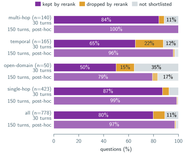
Figure 7: Where T0R’s accuracy stops, by category, on the 778 questions of the five held-out conversations: the rerank kept at least one evidence turn (purple), evidence was in the shortlist but the rerank kept none of it (amber), or no evidence turn was in the shortlist (grey). Upper bar of each pair: T0R’s 30-turn shortlist (shortlist recall, exploratory as registered). Lower, lighter bar: T0R-wide’s 150-turn shortlist (post-hoc). Percentages are printed where the segment is wide enough.
