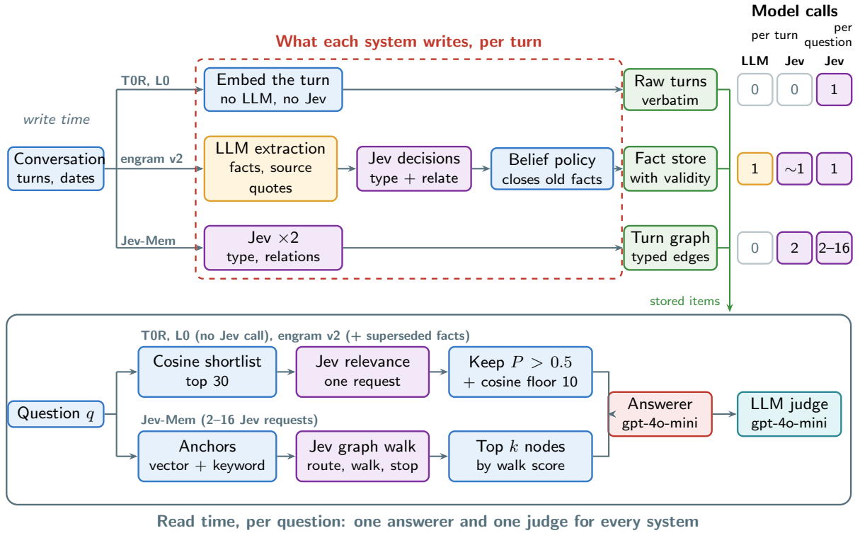
Figure 1: Write path (per turn, top) and read path (per question, bottom) of T0R, L0, engram v2 and Jev-Mem. Border colour says what does the work: code (blue), an LLM call (amber), a Jev typed decision (purple), a store (green), the answer model (red) and the judge (teal). The grid gives LLM calls and Jev requests per turn and Jev requests per question, from each system’s code (Jev-Mem: its default profile). A design diagram; no measured data.
